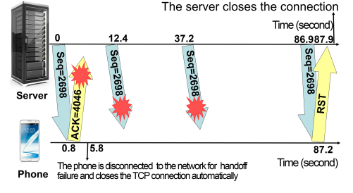
(b) Transmission failure
