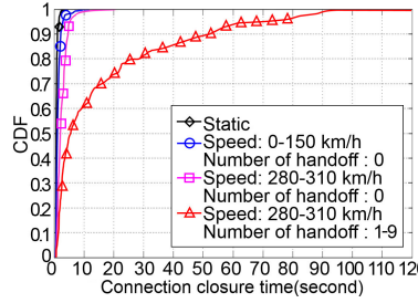
(b) Connection closure
