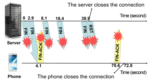
(a) Closure delay
