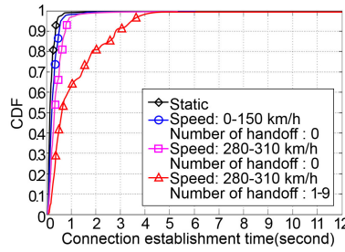
(a) Connection establishment
