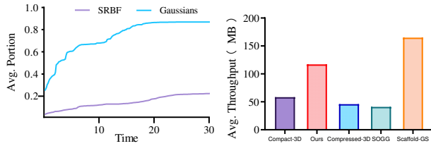
Figure 13: The Avg. Portion of Gaussians and SRBFs after Occlusion Culling.
