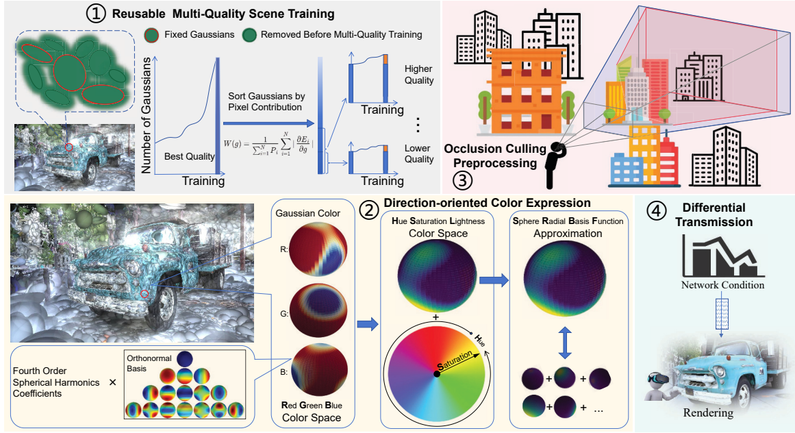
Figure 6: Overview of SRBF-Gaussian.
