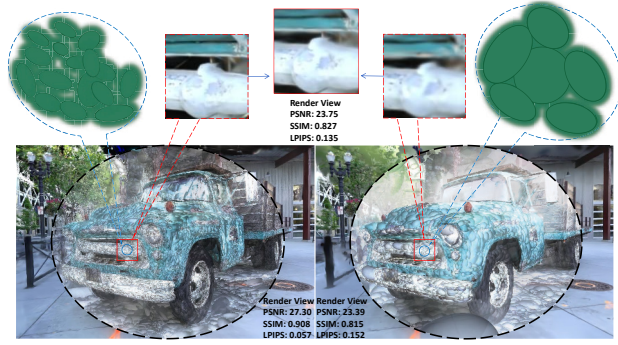
Figure 5: Illustration of the challenges in merging Gaussians of different densities, demonstrating that lower-quality Gaussians are not simply subsets of higher-quality representations.
