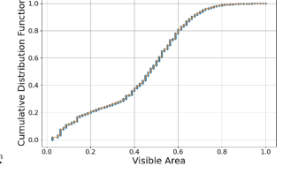
Figure 3: Cumulative Distribution Function of the visible portion of Gaussians in 3DGS.
