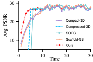
Figure 10: The Avg. value of PSNR over time.
