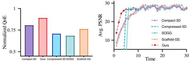
Figure 9: Performance comparison using overall QoE.
