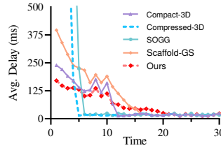
Figure 11: The Avg. latency of baselines over time.
