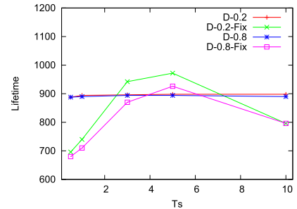
FIGURE 19. Lifetime as a function of T_s for temperature trace.
