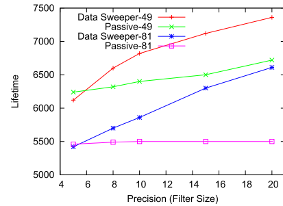
FIGURE 24. Lifetime as a function of precision settings for dewpoint trace with aggregation.
