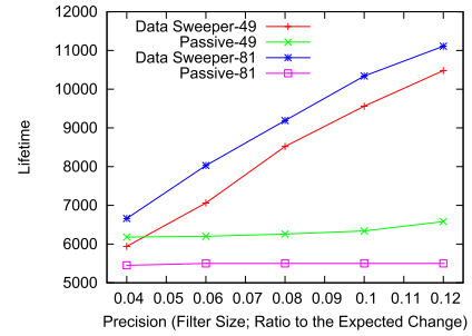
FIGURE 23. Lifetime as a function of precision settings for synthetic data with aggregation.
