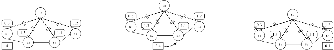
FIGURE 2. An example of the data sweeper scheme. Total user allowed filter size (error bound) is 4. Data readings are shown above the sensor nodes and filters are shown below the sensor nodes. Node s_0 is the base station. Only part of the network is shown, and the dashed lines with interruption represent multi-hop network connections. (a) Data sweeper with whole filter size. (b) Data sweeper moves and suppresses data reports. (c) All four data reports are suppressed.
