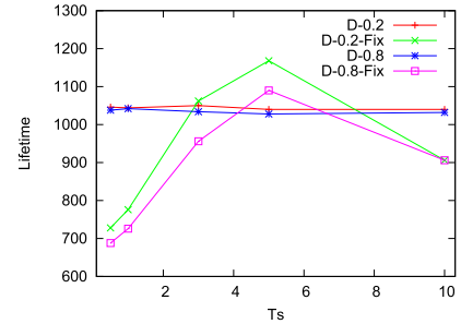
FIGURE 18. Lifetime as a function of T_s for dewpoint trace.
