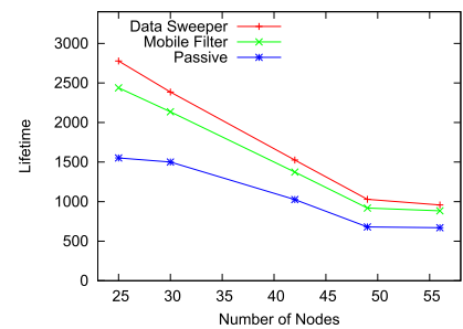
FIGURE 14. Lifetime as a function of the number of nodes for synthetic data.
