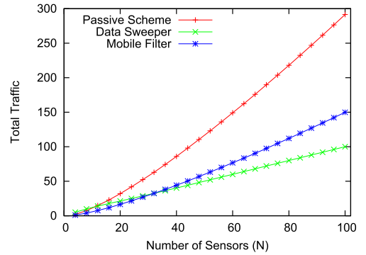
FIGURE 4. Transmission cost as a function of the number of nodes N .
