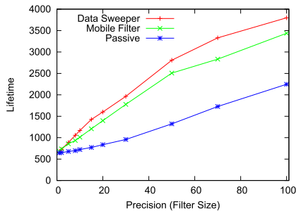
FIGURE 10. Lifetime as a function of precision settings for temperature trace.
