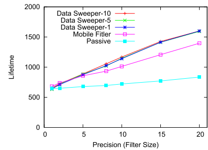
FIGURE 13. Lifetime as a function of precision settings for temperature trace.
