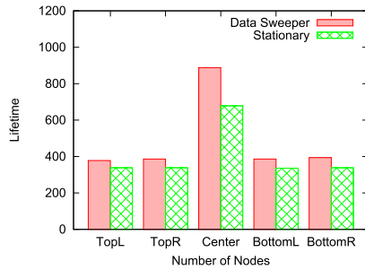
FIGURE 22. Lifetime for different underlying routing topologies for temperature trace.
