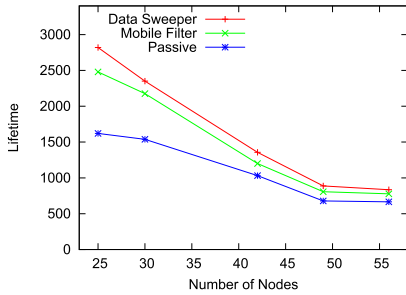
FIGURE 16. Lifetime as a function of the number of nodes for temperature trace.
