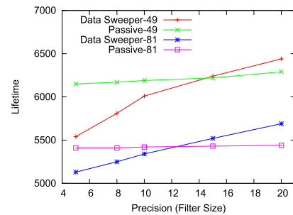
FIGURE 25. Lifetime as a function of precision settings for temperature trace with aggregation.
