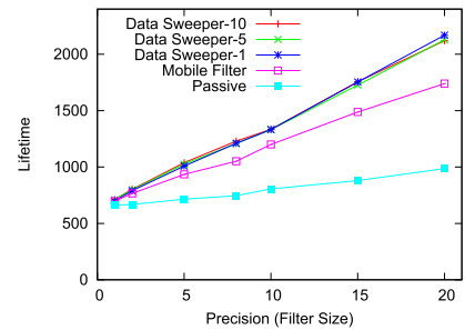
FIGURE 12. Lifetime as a function of precision settings for dewpoint trace.
