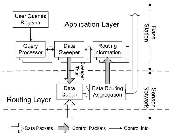
FIGURE 3. Data Sweeper framework.
